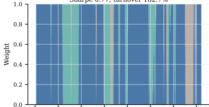
Smoothing half-life 0 Sharpe 0.77; turnover 182.7%
