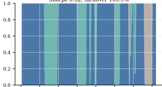
Smoothing half-life 3 Sharpe 0.52; turnover 105.9%
