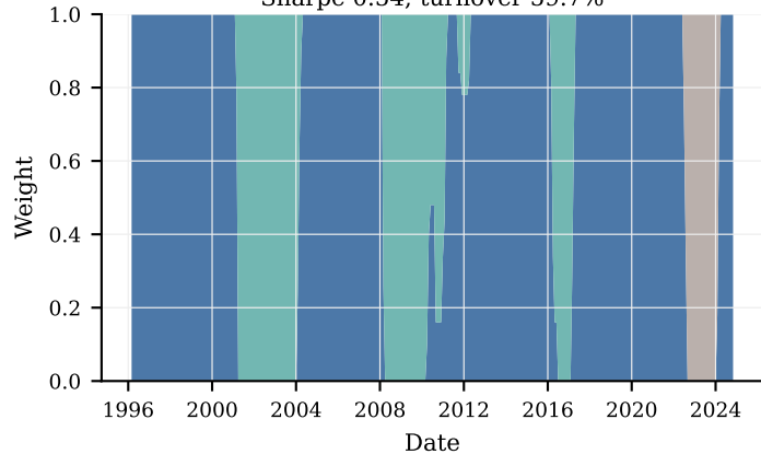
Smoothing half-life 6 Sharpe 0.54; turnover 59.7%
